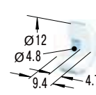
尼龙冲击头 W 3 max = 14 Nm
